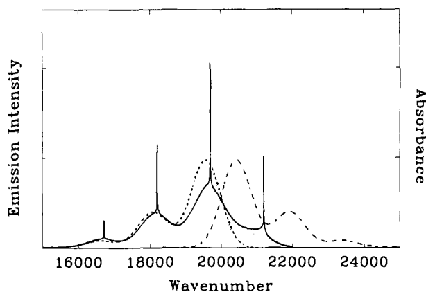
Figure 4. Absorption (long dashes), relaxed emission (short dashes), and unrelaxed emission (solid) spectra using the Brownian oscillator model at an excitation energy of 21 200 \text{cm}^{-1} . All other parameters are as in Figure 1.
