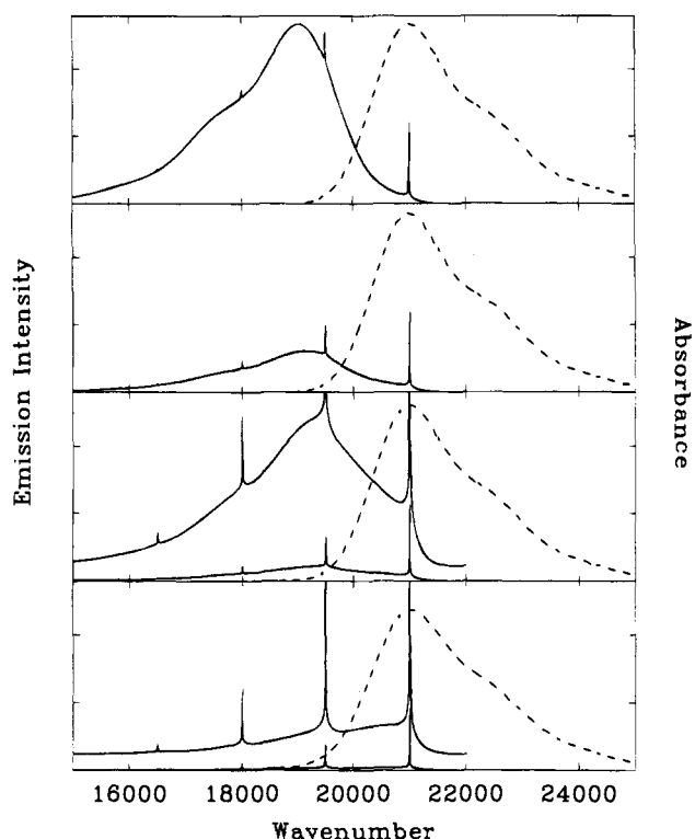
Figure 5. Absorption (dashed) and unrelaxed emission (solid) spectra as a function of excited-state lifetime using the Brownian oscillator model for the solvent with \Delta_S/2\pi c = 648 \text{cm}^{-1} , \Lambda/2\pi c = 64.8 \text{cm}^{-1} , and excitation at 21 000 \text{cm}^{-1} . From top to bottom, \gamma_{ba}/2\pi c = 3, 12, 30, and 120 \text{cm}^{-1} , respectively. All other parameters are as given in Figure 1. Emission spectra are shown both on a common intensity scale and expanded by a factor of 10 in the bottom two panels.
